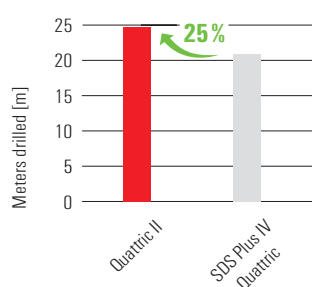
Service life in concrete*
