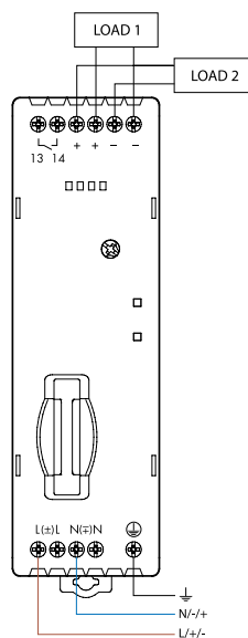
78.1D - Power supply connection
