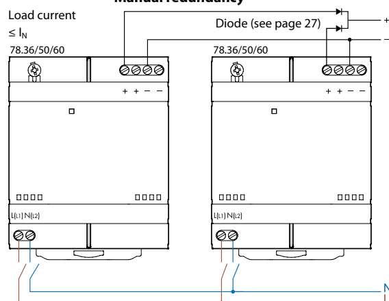
Manual redundancy
