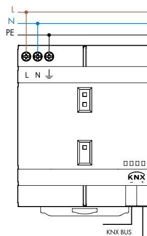
Wiring diagram for 78.2K
