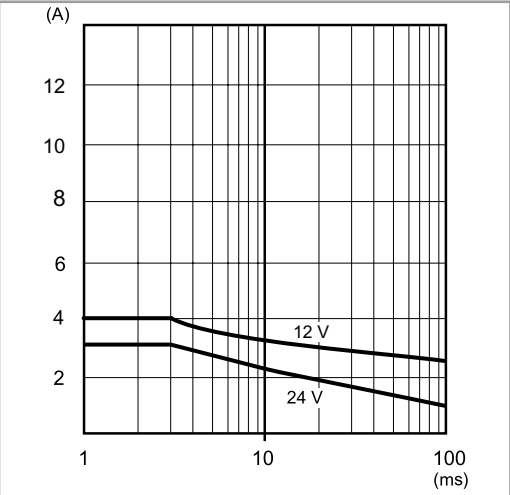
P78-3 Output peak current v time (78.36) - 12 V
