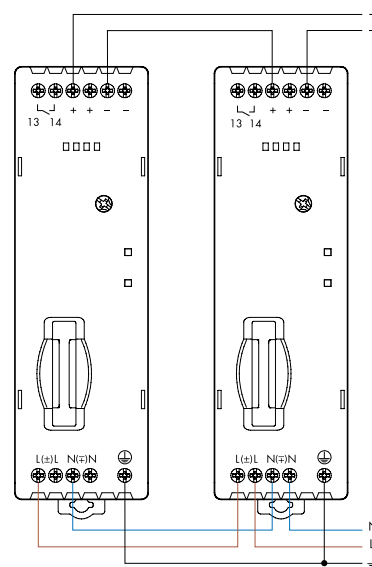
Series connection
