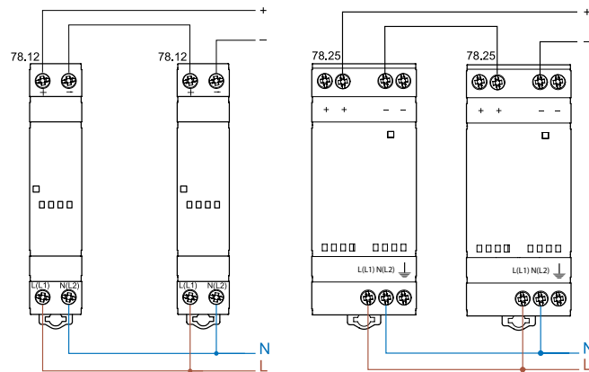
Series connection
