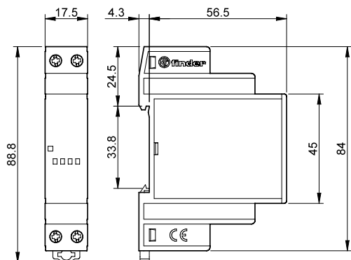
Type 78.25 Box clamp
