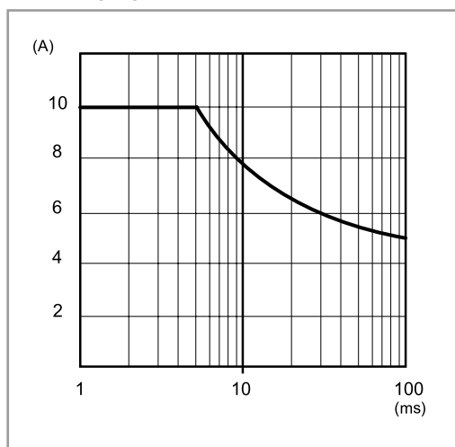
P78-9 Output peak current v time (78.1D)
