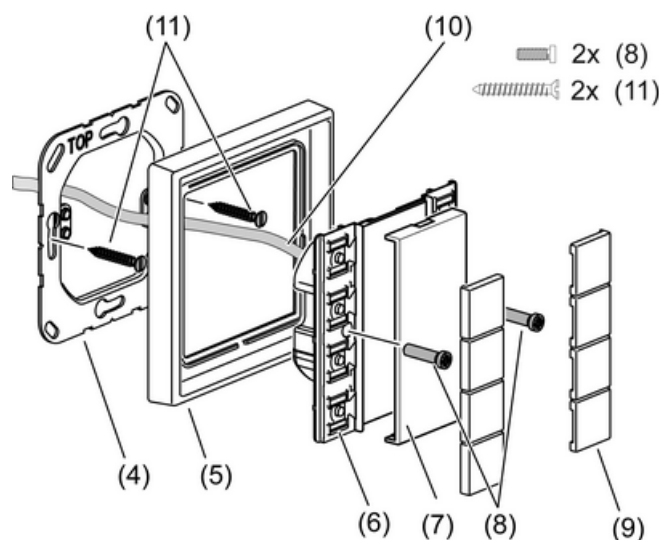
Figure 2: Example of 4-gang push-button module installation
