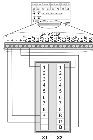
Figure 3: Connection example of channel 1 with status LED and blue operation LED
