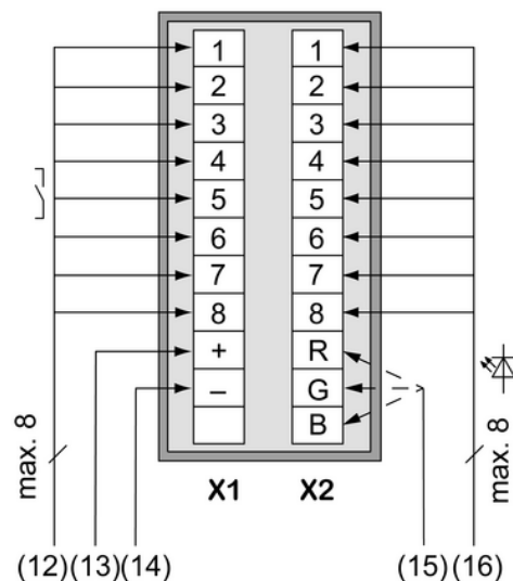
Figure 4: Wiring example for 4-gang push-button module
